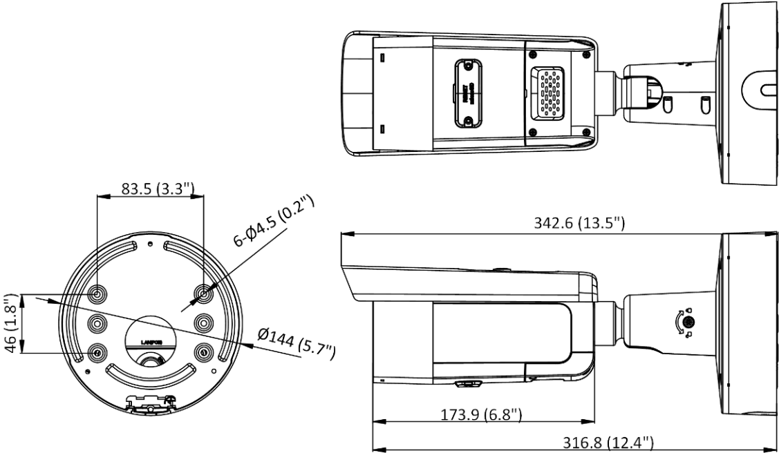
Unit: mm (inch)
