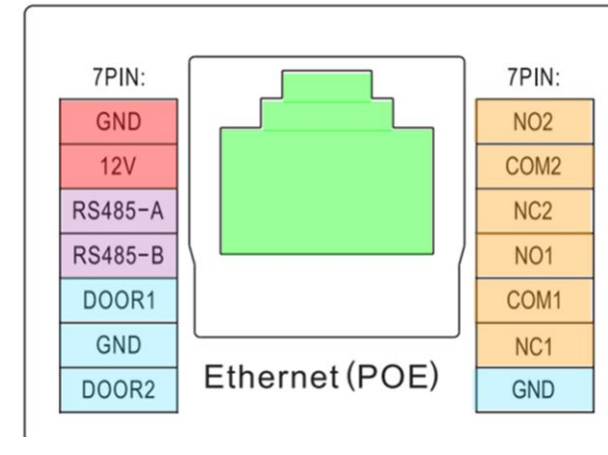
Figure 1.2-1 R26's interface
