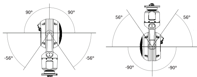
Tilt range of MIC IP fusion 9000i camera
