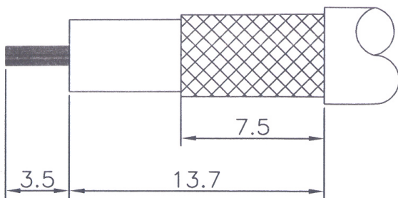
4. Recommended cable stripping lengths
