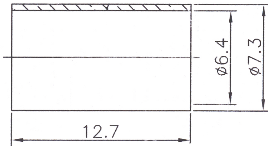
3. Outer Sleeve
