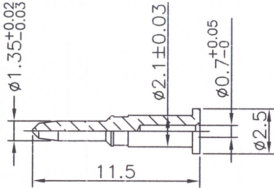
2. Central Pin
