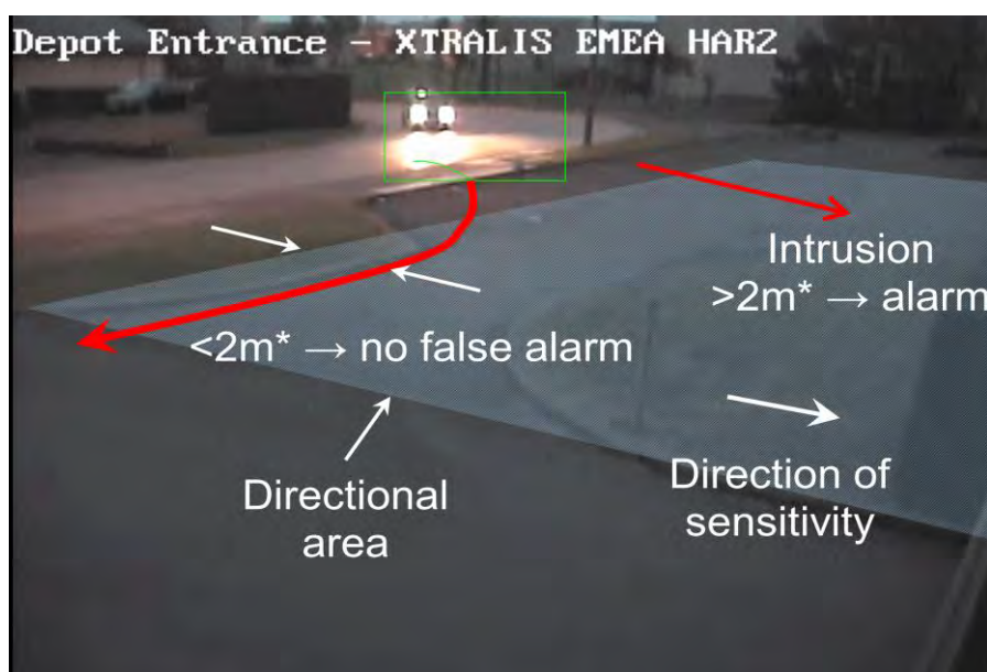
Figure 22: The use of a directional area to filter these false alarms where 2m is set by the minimum distance setting in the advanced configuration
