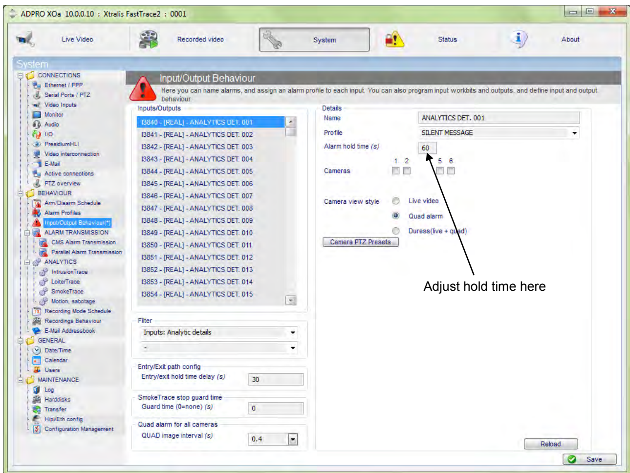
Figure 35: Example showing the hold time for Analytics Detection event 001 being set to 60s
