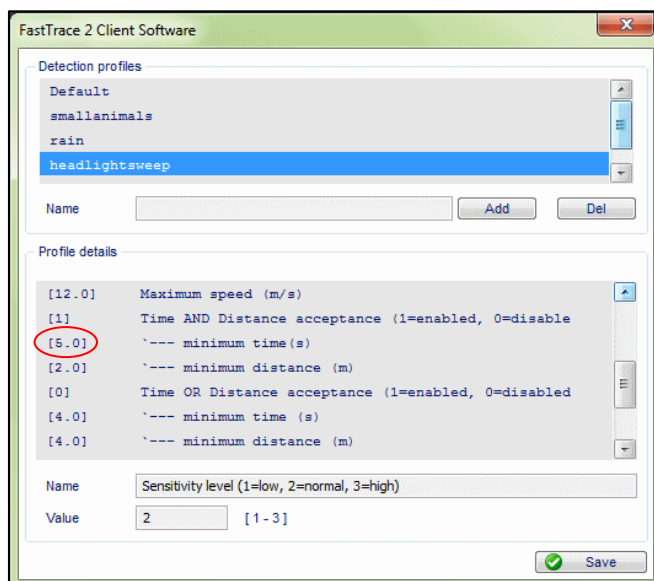
Figure 19: Advanced Settings for Sweeping Headlight Filtering
