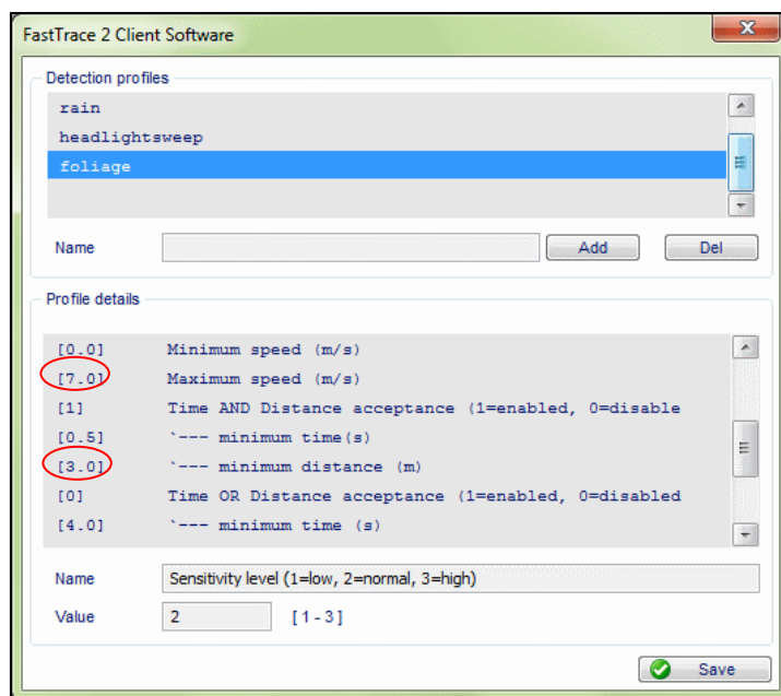
Figure 25: Advanced Settings for Moving Foliage Suppression
