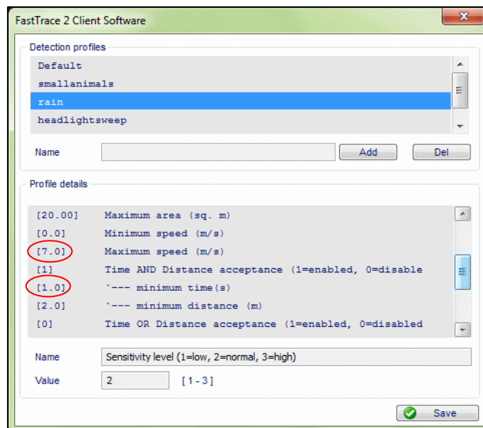
Figure 17: Advanced Settings for Rain and Snow Filtering
