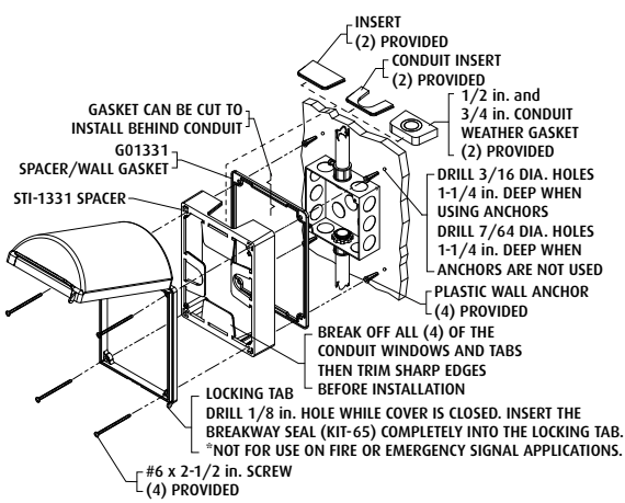
Fig. 3 - Flush Mount with add-on Spacer - Models 131** & 141**
