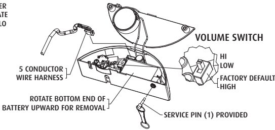
Fig. 7 - Horn Option Models STI-13x20 & STI-13x30 - Wiring Details - Remote Power/Relay Options
